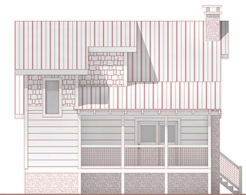
Left Elevation
