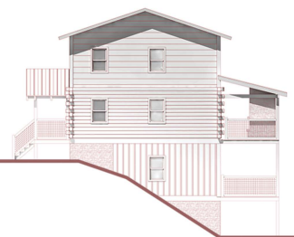
Left Elevation
